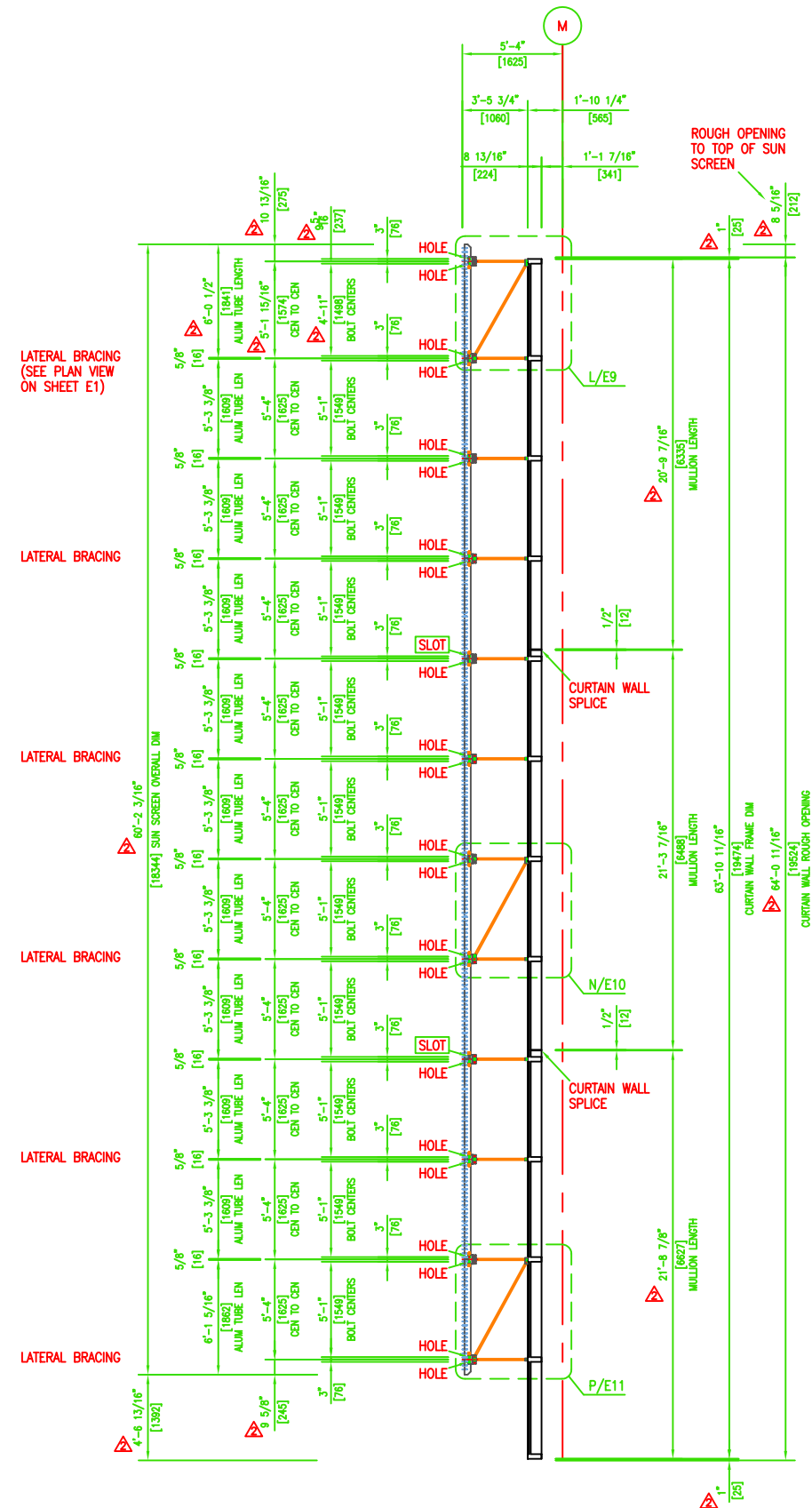
R SECTION THRU SUN SCREEN SCALE 1/8" = 1'-0"
