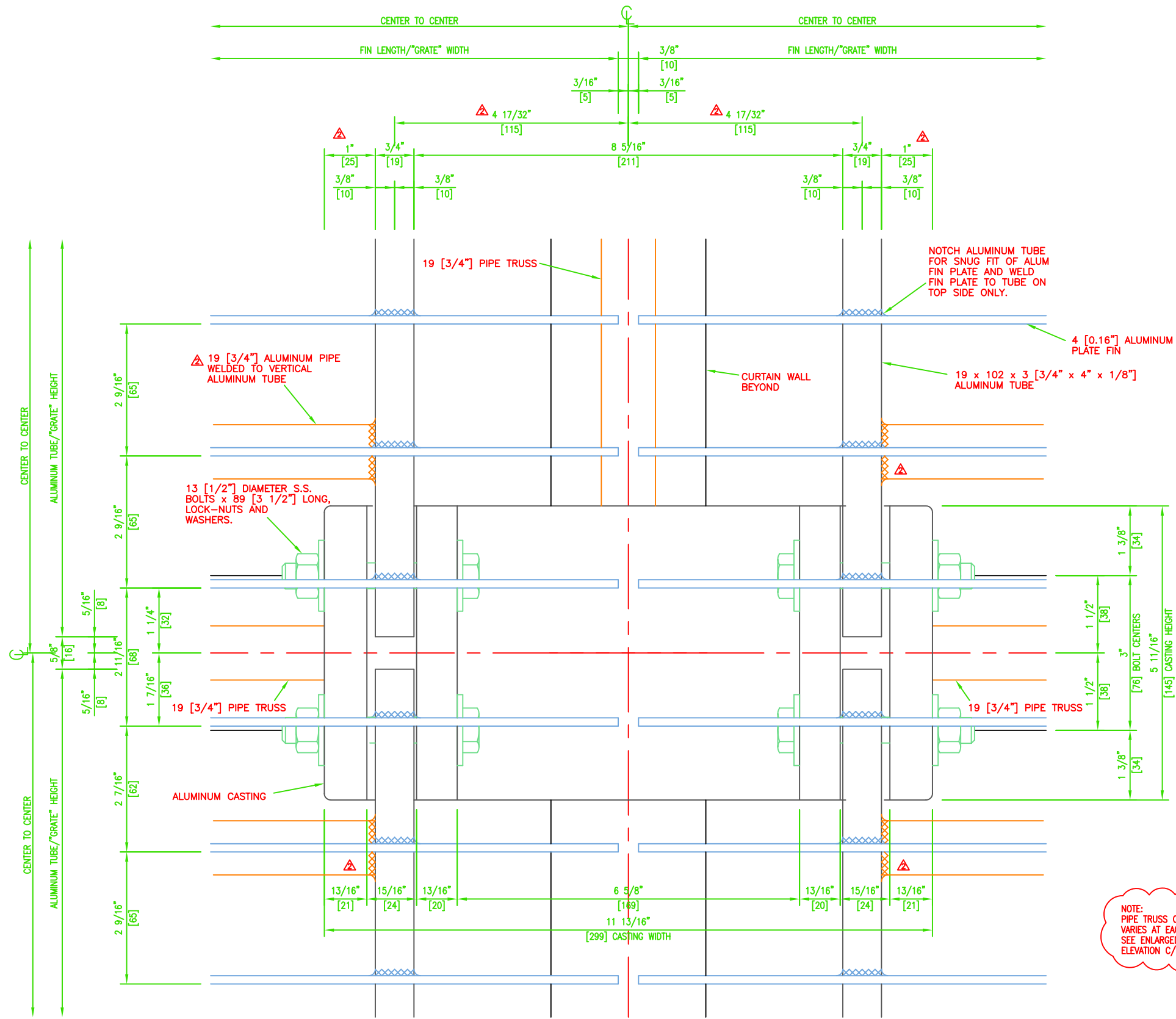
14 FRONT VIEW OF CASTING SCALE 6"=1'-0" REF: ---/--
